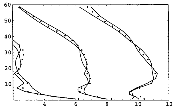
Figure 5. Vertical profiles, triplets at 6, 42, and 71 °N, for each reaction, of the concentration of HONO that would exist if reactions #20, #21, and #22 of Table 2 were in chemical equilibrium with ambient reactants and products of reactions: (left) 2\text{NO}_2 + \text{H}_2\text{O} = \text{HONO} = \text{HNO}_3 ; (middle) \text{NO} + \text{NO}_2 + \text{H}_2\text{O} = 2\text{HONO} ; (right) \text{HNO}_3 + \text{NO} = \text{HONO} + \text{NO}_2 .
