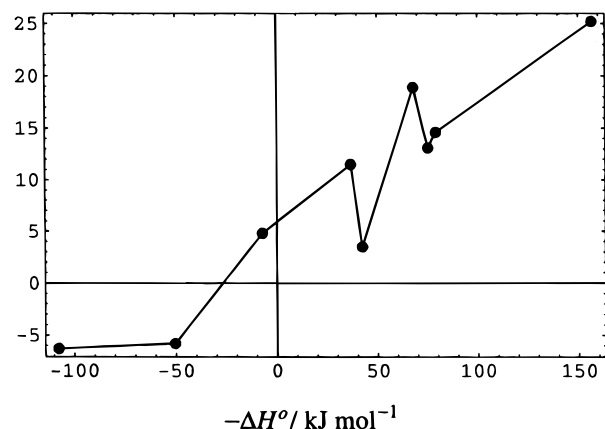
Figure 4. Plot of \log(K/Q) as a function of negative heat of reaction ( -\Delta_r H^\circ/\text{kJ mol}^{-1} ) for the nine reactions in Table 1 with no change in number of gas molecules between reactants and products ( \Delta_r n = 0 ).
