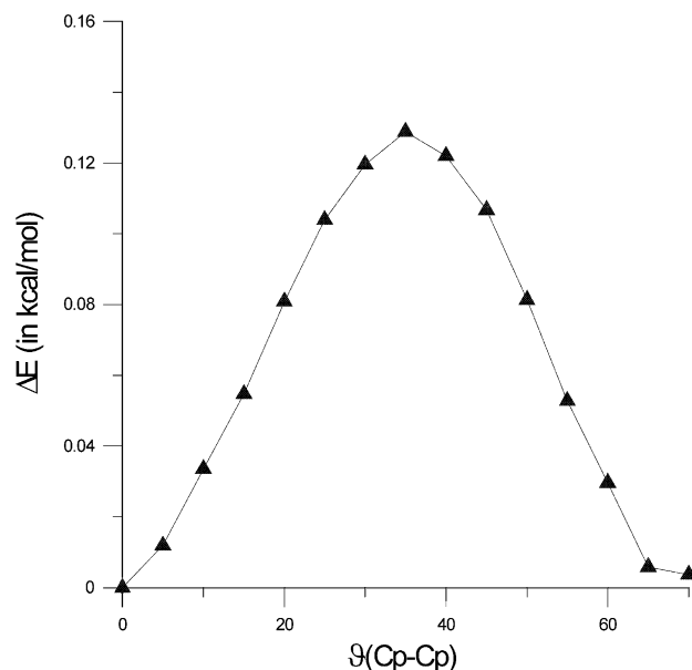
Fig. 7. D_{5h} \rightarrow D_{5d} rotational barrier for ferrocene ( 1 ) (B3LYP/6-31G*).
