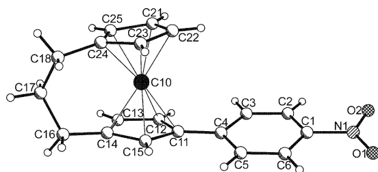
Fig. 1. Crystal structure of compound 4.
