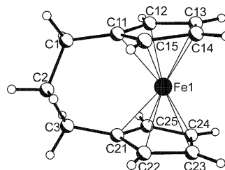
Fig. 8. Crystal structure of [3]ferrocenophane ( 3a ).
