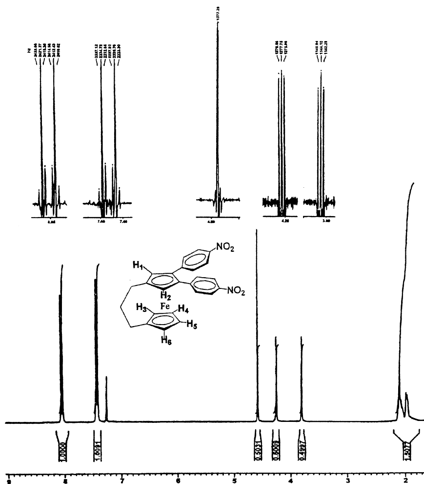
Fig. 6. ^1\text{H} -NMR spectrum of compound 7.
