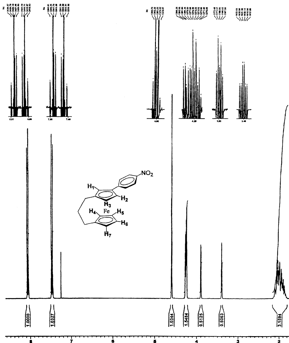
Fig. 2. ^1\text{H} -NMR spectrum of compound 4 .
