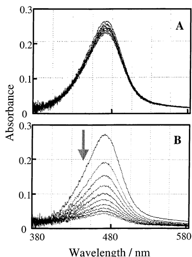
Figure 4. Changes in absorption spectra observed after mixing of the AN solution of 0.10 mM TBPA \bullet^+ with the AN solution of DMT. [DMT]: (A) 0.10 mM and (B) 1.0 mM. Time interval of each spectrum: 1.0 s. Composed of 10 spectra. While DMT \bullet^+ is almost stable without DMT as in A, monotonic decrease of DMT \bullet^+ was observed in the reaction of 0.05 mM DMT \bullet^+ with 0.45 mM DMT as shown in B.
