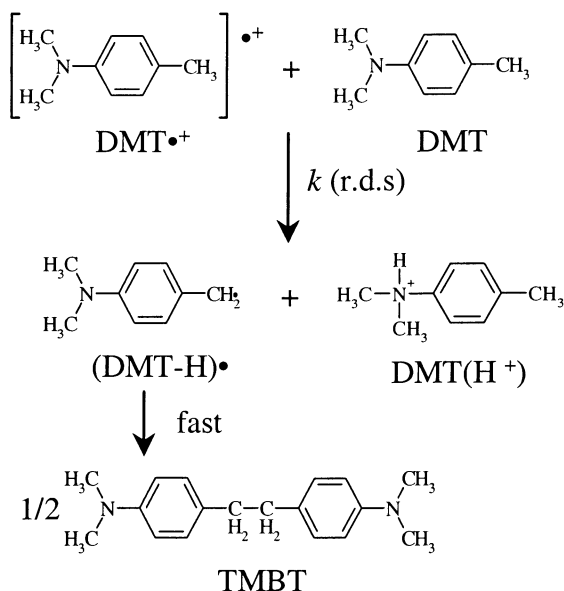
Figure 9. Mechanism of the dimerization reaction of DMT \bullet^+ with the presence of DMT.
