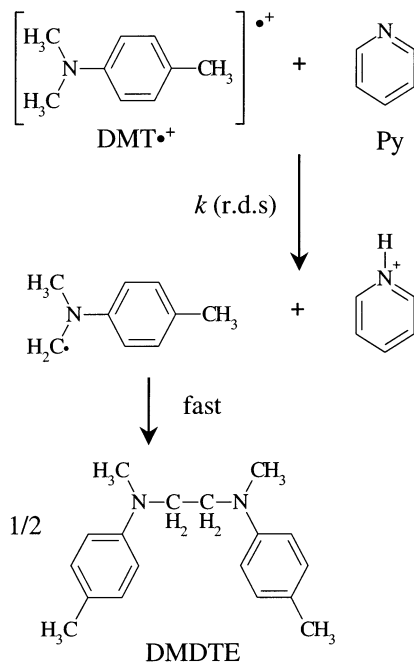
Figure 10. Mechanism of the dimerization reaction of DMT \bullet^+ with the presence of Py.
