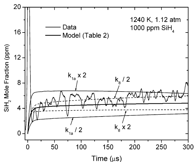
Figure 9. Effects of uncertainties in k_{1a} and k_8 on the present measurements of \text{SiH}_2 concentration.
