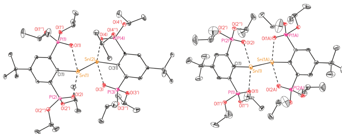
Figure 1. Molecular structure of compound 2 in the crystal of 2 (left) and in the crystal of 2 ·C 7 H 8 (right) (ORTEP presentation at 30% probability of the depicted atoms). H atoms are omitted for clarity. The toluene molecule was removed by PLATON/SQUEEZE. 19 Symmetry code: A) 0.5 – x , 0.5 – y , 1 – z .
