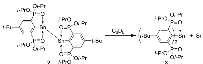
Scheme 2. Disproportionation of Compound 2 To Give Elemental Tin and the Diorganostannylene 3
