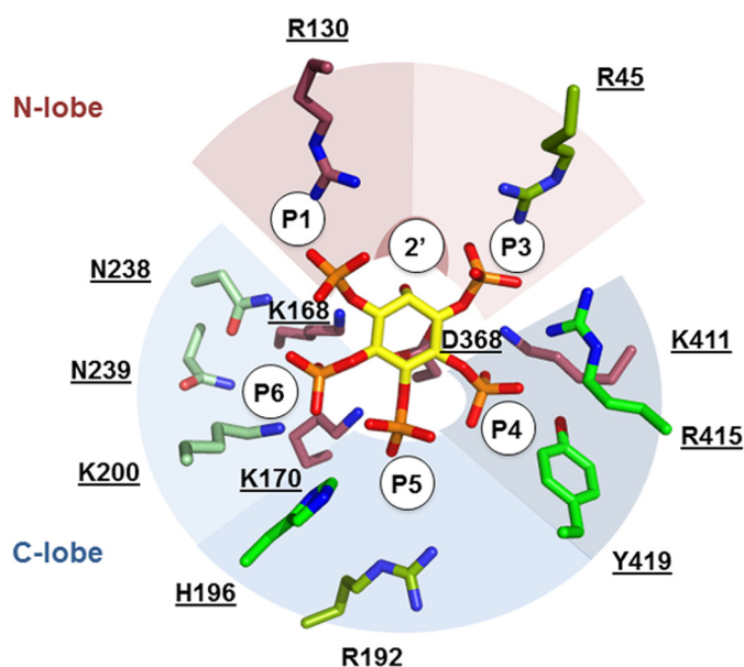
FIGURE 2. Structural representation of kinetic parameters of alanine mutants. IP 5 is shown in yellow stick form. The side chains of IP-binding residues are shown in stick form and colored according to alanine mutant k_{cat} . Maroon indicates no activity. Darker green shades indicate reduced activity compared with wild-type IPK1. Green indicates equivalent activity to wild-type IPK1. Side chains are grouped according to bound phosphate, overlaid with colored arcs (red, N-lobe; blue, C-lobe).
