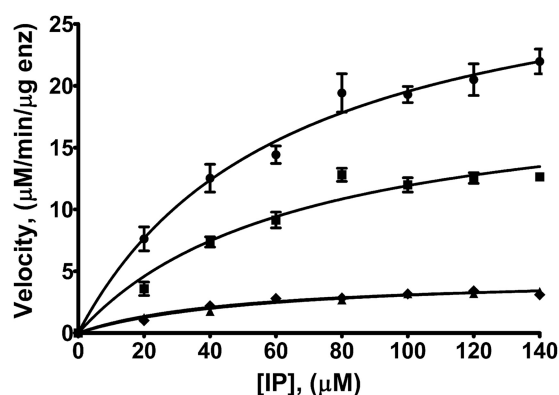
FIGURE 1. Kinetic analysis of the kinase activity of IPK1 for IP_5 and IP_4 s. IPK1 kinase activity was assessed using a luminescence-based assay. The rate of product formation versus IP concentration was plotted and fitted to the Michaelis-Menten equation. Each point represents the mean \pm S.D. of triplicate experiments. \bullet , IP_5 ; \blacksquare , 1,3,4,6- IP_4 ; \blacklozenge , 3,4,5,6- IP_4 ; \blacktriangle , 1,4,5,6- IP_4 . enz, enzyme.
