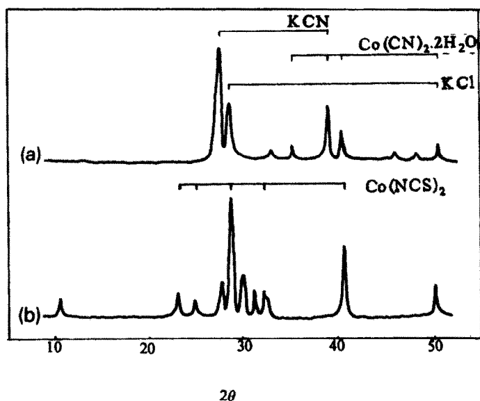
Fig. 3. XRD results for solid products in a hydrogen atmosphere: (a) 300°C, [\text{Co}(\text{NH}_3)_6]\text{Cl}_3 + \text{KCN} ; (b) 200°C, [\text{Co}(\text{NH}_3)_6]\text{Cl}_3 + \text{KSCN} .
