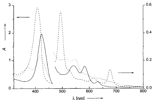
Figure 2. UV/Vis spectra of nickel oxaporphyrin complexes. Solid line = [(\text{ODTDPP})\text{Ni}^{\text{II}}\text{Cl}] (dichloromethane), dashed line = [(\text{O}_2\text{TPP})\text{Ni}^{\text{II}}\text{Cl}_2] (dichloromethane), dotted line = [(\text{ODTDPP})\text{Ni}^{\text{II}}] (benzene).
