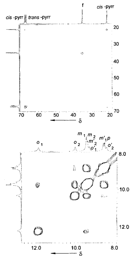
Figure 4. The 2D ^1\text{H} COSY spectrum of [(\text{ODTDPP})\text{Ni}^{\text{II}}\text{Cl}] ( \text{CDCl}_3 , 273 K). Upper map: lowfield region showing spin–spin coupling of regular pyrrole protons; lower map: meso-phenyl region. Peak labels: trans -pyrr and cis -pyrr denote 7,8,17,18- and 12,13- pyrrole protons, respectively; f: furan; o , m , p denote resonances of ortho , meta , or para protons of 10,15-phenyl rings; o' , m' are assigned to ortho and meta protons of 5,20- p -tolyl groups.
