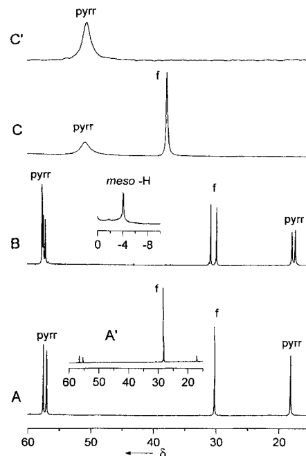
Figure 3. NMR spectra (293 K) of: A) [(\text{ODTDPP})\text{Ni}^{\text{II}}\text{Cl}] ( \text{CDCl}_3 , ^1\text{H} NMR); A') [(\text{D}_4\text{O}_2\text{TPP})\text{Ni}^{\text{II}}\text{Cl}] ( \text{C}_6\text{D}_6 , ^1\text{H} NMR); B) [(\text{OPDTP})\text{Ni}^{\text{II}}\text{Cl}] ; C) [(\text{O}_2\text{TPP})\text{Ni}^{\text{II}}\text{Cl}_2] ( \text{CDCl}_3 , ^1\text{H} NMR); C') [(\text{D}_4\text{O}_2\text{TPP})\text{Ni}^{\text{II}}\text{Cl}_2] ( \text{CHCl}_3 , ^2\text{H} NMR). Peak labels: pyrr: pyrrole ring protons; meso-H: 5-CH; f: furan.
