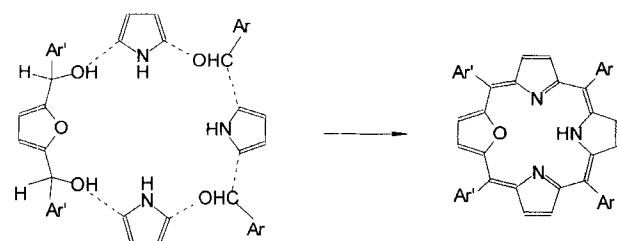
Scheme 3. Synthetic route to 21-oxatetraphenylporphyrin.
