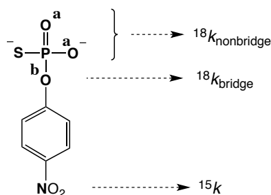
Figure 3. The substrate p NPPT ( 2a ) with the positions indicated at which isotope effects were measured.
