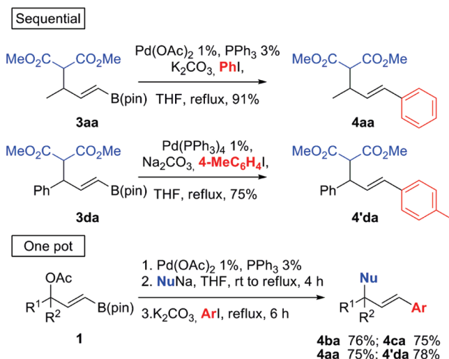
Scheme 2. One-Pot Tsuji–Trost Suzuki–Miyaura Reaction
