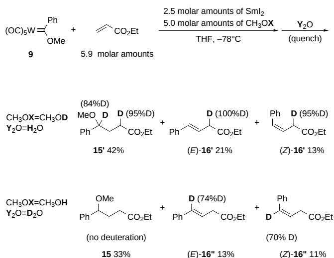
Scheme 7. Deuterium-labeling experiments.
