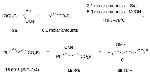
Scheme 15. Reaction of phenylcarbene complex of chromium 35 .
