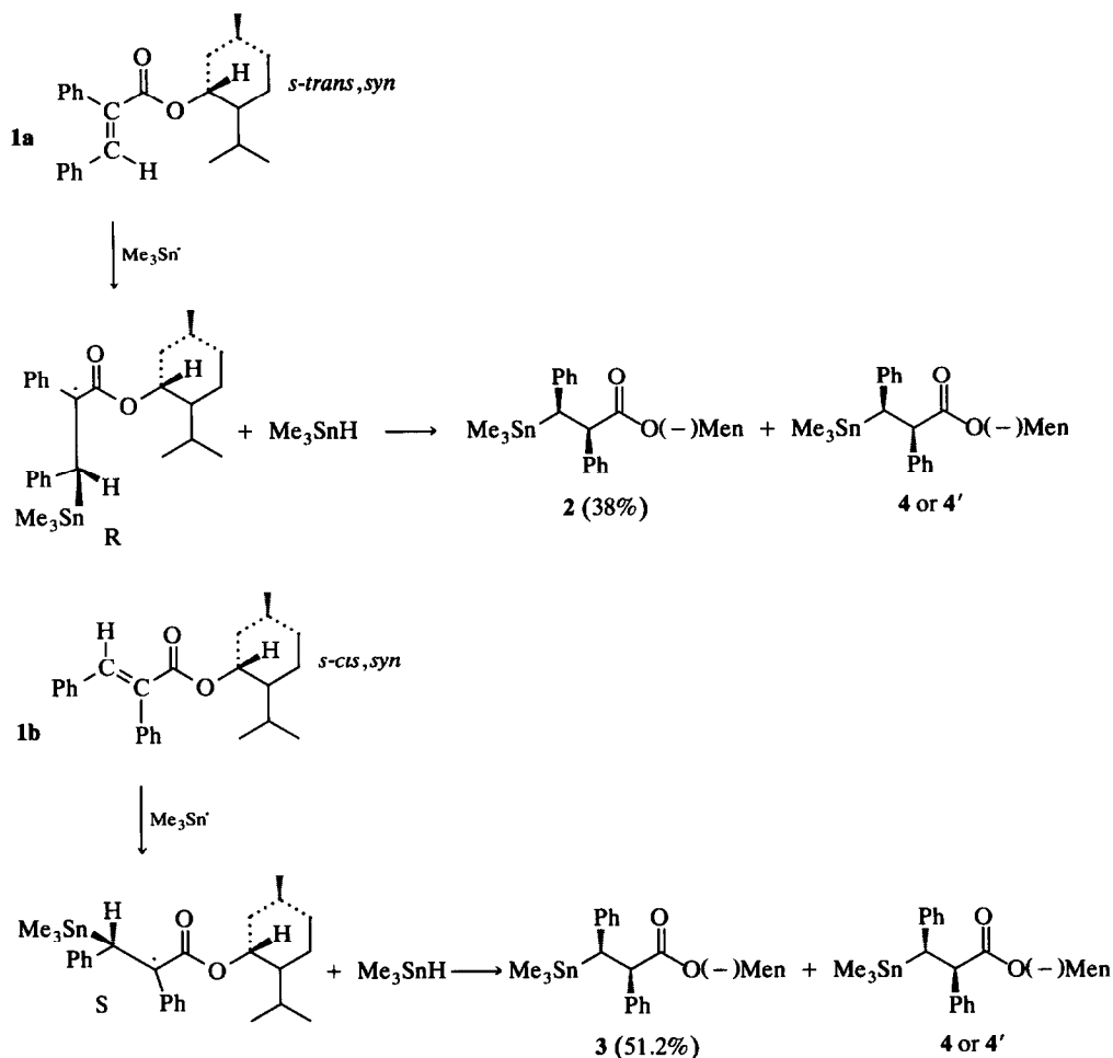
Scheme 6. Stereochemistry of hydrostannation of the s-trans,syn and s-cis,syn conformations of (–)-menthyl ( E )-2,3-diphenylpropenoate ( 1a and 1b ) with trimethyltin hydride.
