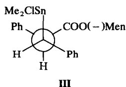
Fig. 2 Preferred conformations for compounds 5 and 6 (one stereoisomer is shown).
