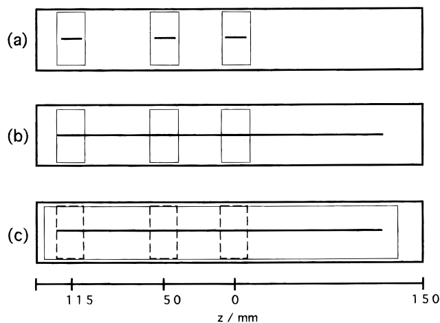
Figure 2. Experimental setup for size effects of chromatography paper and copper wire on the yield of copper ions. (a) Small pieces of copper wire (6 \phi \times 15 mm) were placed on small pieces of the paper (37 mm \times 20 mm) at z = 0, 50 , and 115 mm. (b) A copper wire (6 \phi \times 250 mm) was placed on pieces of the paper (37 mm \times 20 mm) at the same positions. (c) A copper wire (6 \phi \times 250 mm) was placed on a long piece of the paper (37 mm \times 300 mm). In cases a and b the relative concentration of copper ions was determined at each piece of paper in the absence and presence of a magnetic field ( B_{\max} = 8 T). In the case of c, after the reaction the paper was cut as indicated by broken lines in the figure, and then the copper concentrations were determined analogously.
