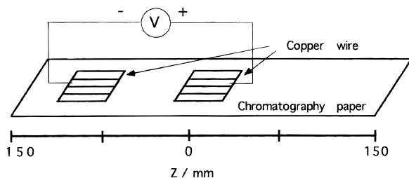
Figure 3. Experimental setup for the electromotive force. Two sets of copper wire (6 \phi \times 50 mm \times 4) were placed on a piece of chromatography paper at z = 0 and z = 125 mm.
