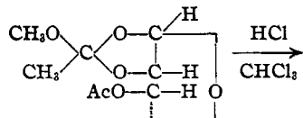
Methylglycoside acetate with an orthoester structure
