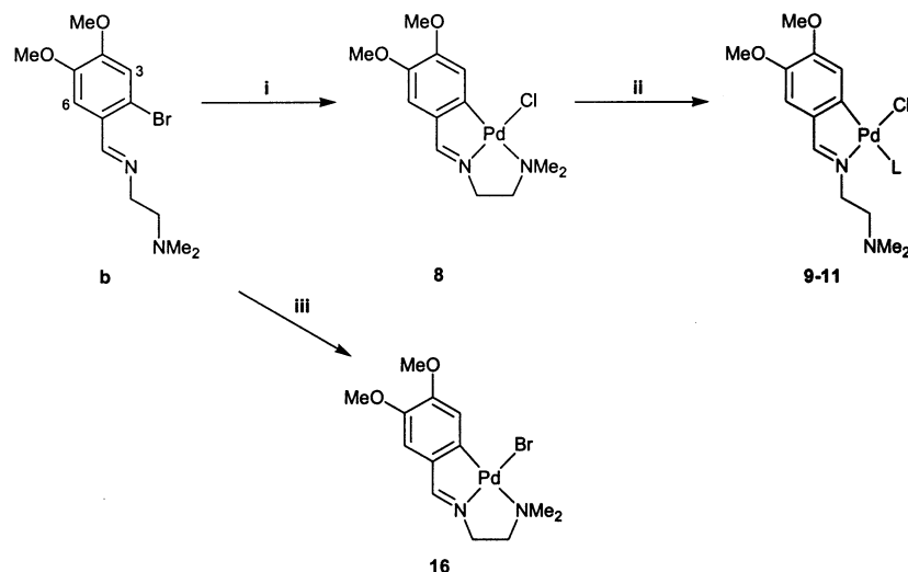
Scheme 2. (i) \text{PdCl}_2 /octane, reflux; (ii) \text{L} /acetone, stir [ \text{L} = \text{PPh}_3 ( 9 ); \text{PEtPh}_2 ( 10 ); \text{PMePh}_2 ( 11 )]; (iii) [\text{Pd}_2(\text{dba})_3] /benzene, reflux.
