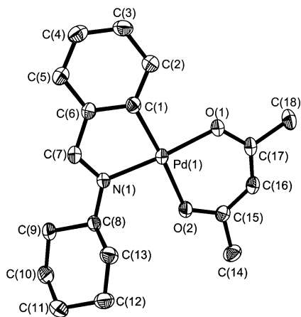
Fig. 1. Molecular structure of compound [\text{Pd}\{\text{C}_6\text{H}_4\text{C}(\text{H})=\text{NCy}\}(\text{MeCOCHCOMe})] ( 2 ), with labelling scheme (30% probability level). Hydrogen atoms have been omitted for clarity.
