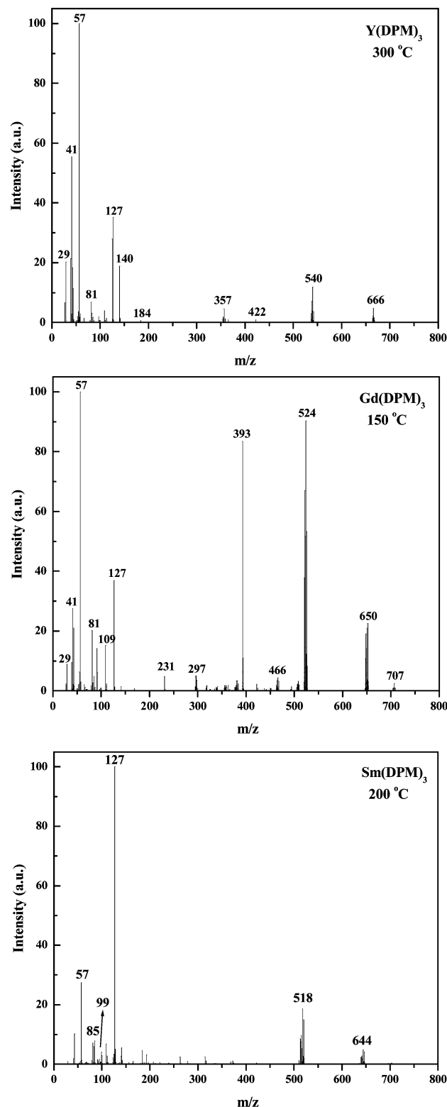
Figure 7. Typical mass spectrum of M(\text{DPM})_3 ( M = \text{Y}, \text{Sm}, \text{and Gd} ).
