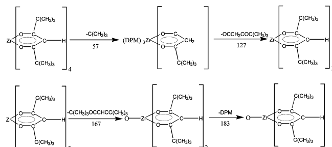
Figure 14. Possible decomposition mechanism of \text{Zr}(\text{DPM})_4 .
