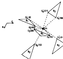
FIG. 2. Neodymium atom environment.
