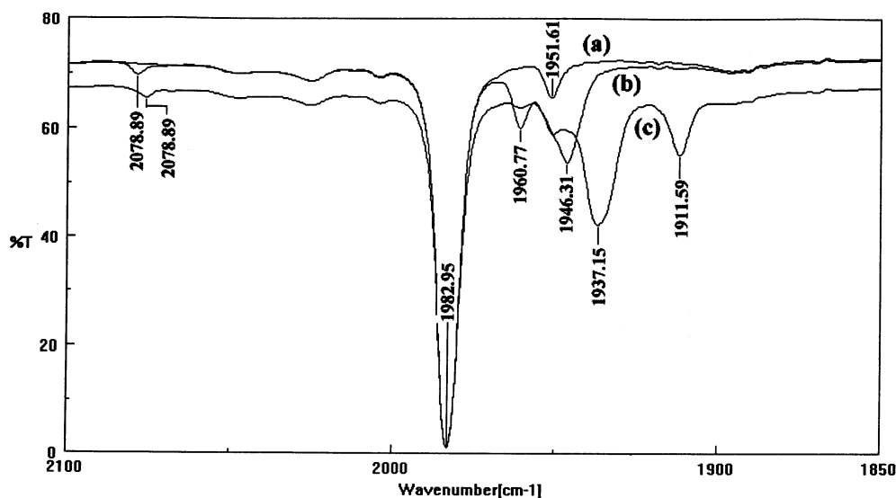
Fig. 2. The changes in the IR spectra of the \text{W(CO)}_6 solution in n -hexane upon irradiation. (a) \text{W(CO)}_6 solution, (b) after photolysis of the solution, (c) after the addition of the cyclohexanone.
