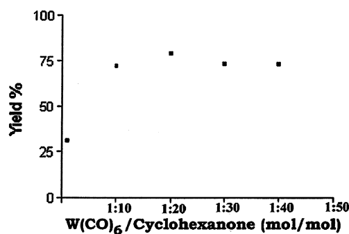
Fig. 1. Variation of the yield of II with the \text{W(CO)}_6 /cyclohexanone ratio:
