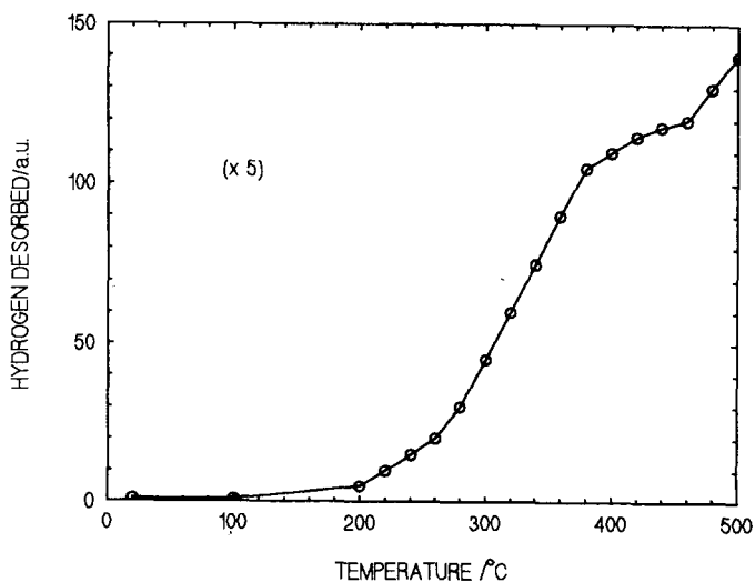
Fig. 5. TPD curve for sample C_3 .
