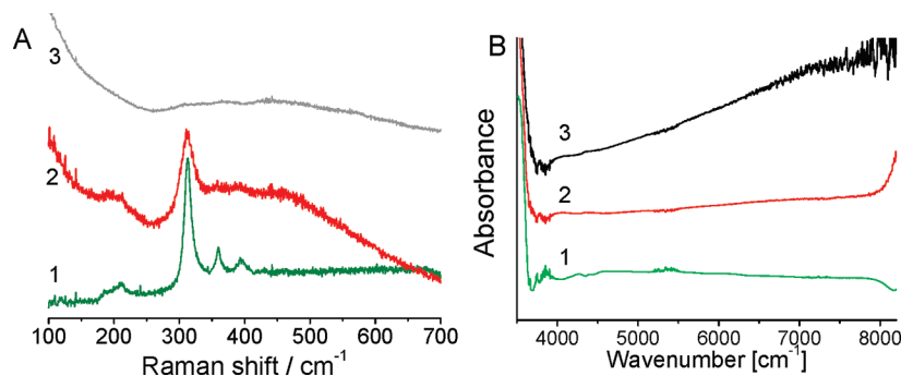
Figure 7. (A) Raman and (B) FTIR spectra of (1) white, (2) red, and (3) black c\text{-In(OH)}_3 at ambient pressure. In (A), the band at 309\text{ cm}^{-1} is attributed to the \nu_3 In–O symmetric stretching vibration, and the bands at 356 and 391\text{ cm}^{-1} are due to the \nu_3 In–O antisymmetric stretching vibrations. 30
