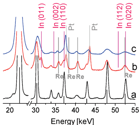
Figure 6. Energy-dispersive XRD patterns of c\text{-In(OH)}_3 in a DAC at ambient pressure: (a) initial sample; (b) black sample recovered after the second experiment; (c) reddish sample recovered after the first experiment. At the bottom of the figure, the diffraction pattern of c\text{-In(OH)}_3 (PCPDFWIN 85-1338) is shown. At the top, the diffraction patterns (intensity set to 100% for all reflections) of metallic In (PCPDFWIN 85-1409), metallic Re (PCPDFWIN 89-2935), and Pt (PCPDFWIN 88-2343) are shown.
