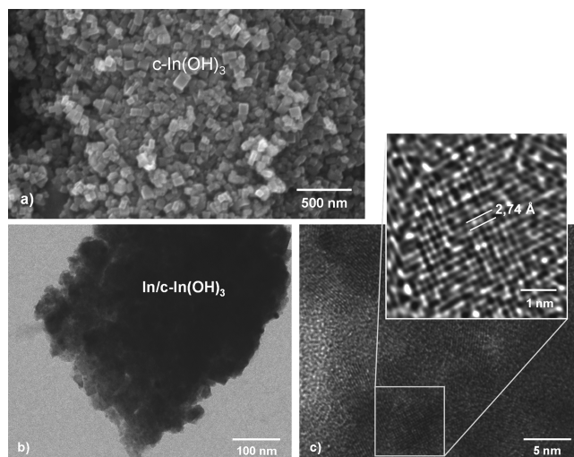
Figure 8. (a) Scanning electron microscopy image of the initial white c\text{-In(OH)}_3 sample. (b, c) TEM micrographs of the recovered black \text{In}/c\text{-In(OH)}_3 sample. The inset in (c) reveals an inverse FFT image of the boxed region. The measured distance obtained from the inverse FFT image is 2.74 Å, which is in good agreement with the d_{011} distance in t\text{-In} .
