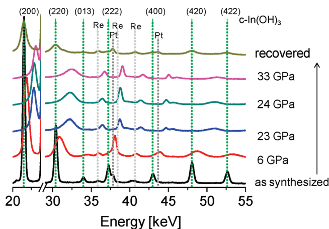
Figure 1. First experiment: in situ energy-dispersive XRD patterns of c-In(OH) 3 in a DAC at different pressures. The label “as synthesized” indicates the starting c-In(OH) 3 in the DAC at ambient pressure. Tick marks indicate diffraction reflections of c-In(OH) 3 (PCPDFWIN 85-1338), Re (PCPDFWIN 89-2935), and Pt (PCPDFWIN 88-2343). The horizontal axis is broken to cut off the indium emission lines ( 49 In Kα 1–2 , Kβ 1–3 ). At the top, the (hkl) planes of c-In(OH) 3 are indicated.
