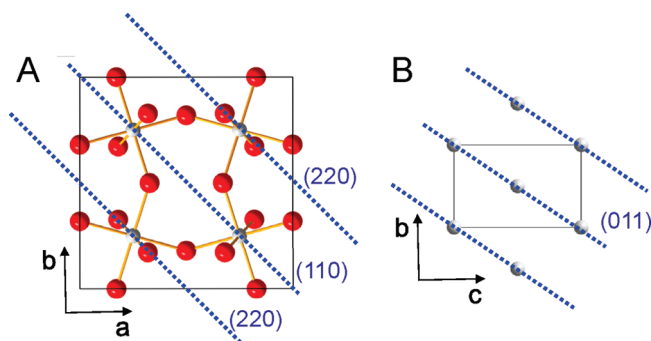
Figure 9. (A) Coordination of indium atoms (small gray circles) by oxygen (large red circles) and interconnection (sharing) of [\text{InO}_6] octahedra in the c\text{-In(OH)}_3 structure under ambient-pressure conditions. The \{220\} planes composed of In atoms are also shown. (B) \{011\} planes in tetragonal indium.
