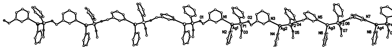
Figure 4. View of the chain of \text{PCP-32AgBF}_4 , 3 , perpetuated in one dimension. The partial spiral of the pyridyl linkages can be seen to abruptly restart at the end of the unique portion. H atoms have been removed for clarity.
