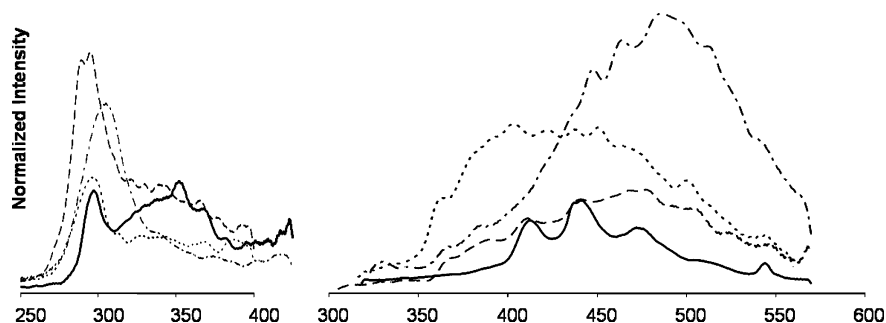
Figure 10. Normalized excitation and emission spectra of compounds 1–4 taken in acetonitrile glasses at 1 \times 10^{-4} M at 77 K: (—) PCP-32, (---) PCP-32AgBF 4 , (···) PCP-32AgOTf, (- · -) PCP-32Ag(tfa).
