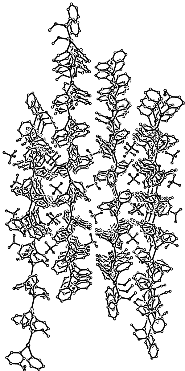
Figure 5. View down the a axis of how the 2-D sheets of \text{PCP-32AgBF}_4 stack together encompassing the \text{BF}_4^- anions. H atoms have been removed for clarity.
