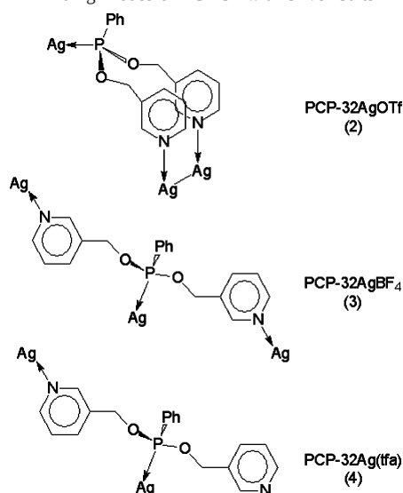
Scheme 2. Binding Modes of PCP-32 with Silver Salts
