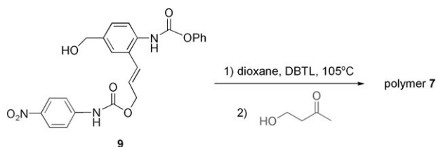
Scheme 4. Synthesis of self-immotive comb-polymer 7 .
