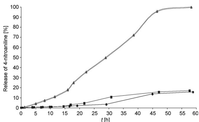
Figure 3. Disassembly (▲) of self-immotive comb-polymer 7 upon treatment with piperidine/AcOH to release 4-nitroaniline. Polymer 7 without treatment of piperidine/AcOH (◆). Polymer 7a upon treatment with piperidine/AcOH (■).
