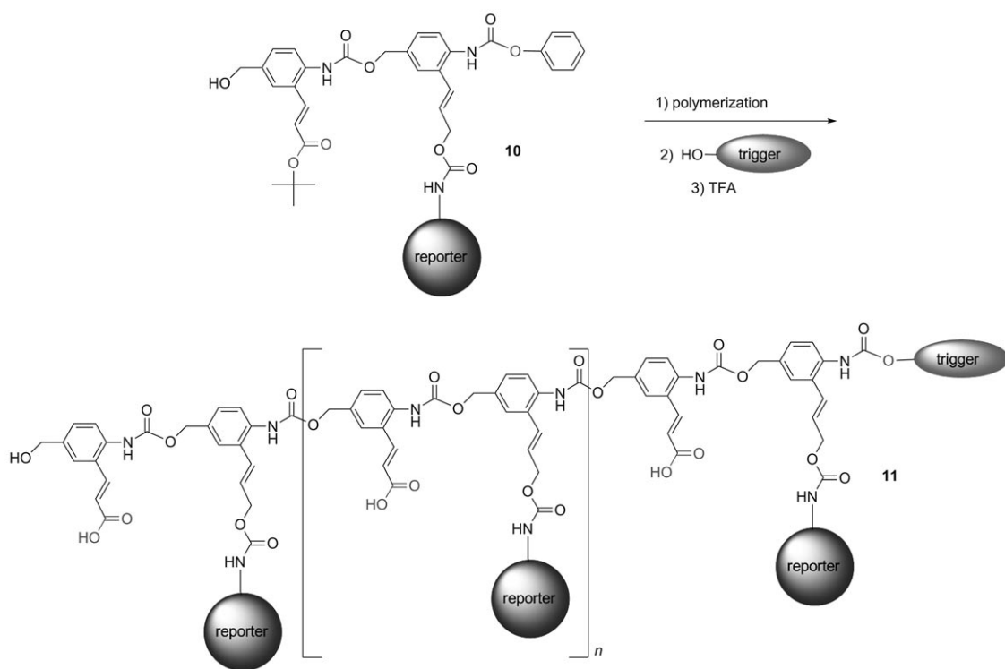
Scheme 5. Synthesis of a water-soluble self-immotive comb-polymer with a trigger.
