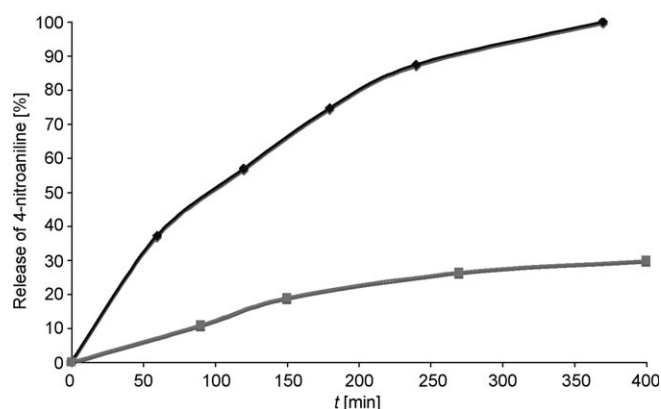
Figure 4. Disassembly (◆) of self-immolative comb-polymer 12 upon addition of PGA to release 4-nitroaniline. Control reaction: polymer 12 in PBS, pH 7.4 (■).
