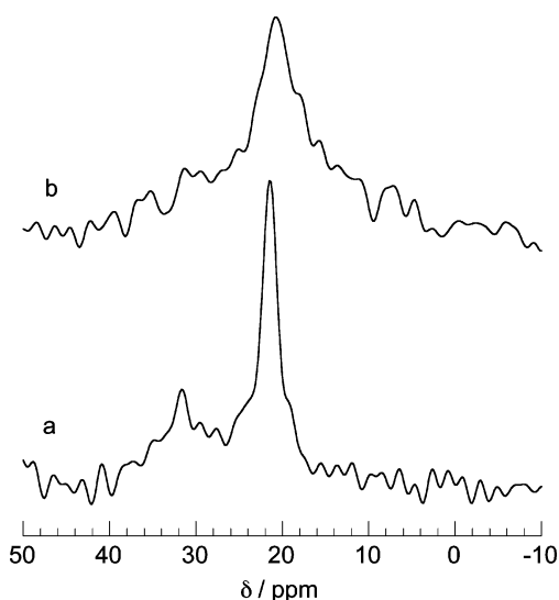
Figure 5. ^{13}\text{C} CP NMR spectra for \text{CH}_3\text{ReO}_3 grafted onto dehydrated silica–alumina (10 wt % Re). Both spectra were recorded at -100^\circ\text{C} , (a) with 8 kHz MAS and (b) without spinning.
