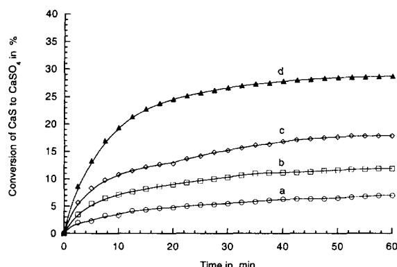
Fig. 2. The effect of temperature on the conversion of CaS to \text{CaSO}_4 for the oxidation of the CaS. Gas composition: 4 vol% \text{O}_2 in \text{N}_2 . Temperature: a – 500°C; b – 750°C; c – 800°C; and d – 865°C.
