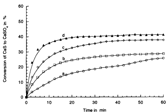
Fig. 4. The effect of \text{O}_2 partial pressure on the conversion of CaS to \text{CaSO}_4 for the CaS oxidation. Temperature: 865°C. Gas composition: a – 1 vol% \text{O}_2 in \text{N}_2 ; b – 4 vol% \text{O}_2 in \text{N}_2 ; c – 20 vol% \text{O}_2 in \text{N}_2 ; and d – 40 vol% \text{O}_2 in \text{N}_2 .
