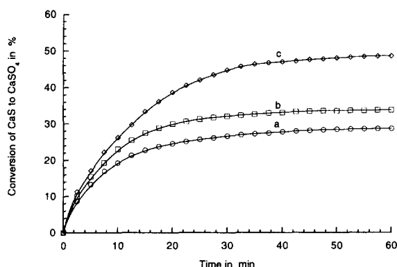
Fig. 3. The effect of particle size on the conversion of CaS to \text{CaSO}_4 during the CaS oxidation. Gas composition: 4 vol% \text{O}_2 in \text{N}_2 . Temperature: 865°C. Particle size: a – 42 µm; b – 30 µm; and c – 17 µm.
