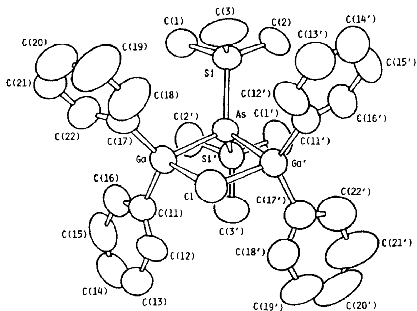
Fig. 1. ORTEP diagram of \text{Ph}_2\text{GaAs}(\text{SiMe}_3)_2\text{Ga}(\text{Ph})_2\text{Cl} ( 1 ) (hydrogen atoms omitted for clarity).
