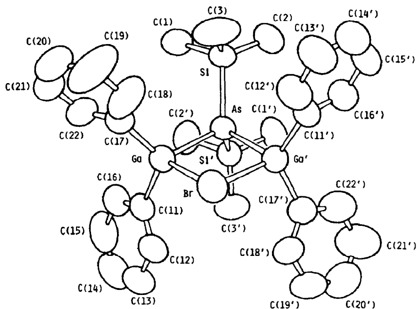
Fig. 2. ORTEP diagram of \text{Ph}_2\text{GaAs}(\text{SiMe}_3)_2\text{Ga}(\text{Ph})_2\text{Br} ( 2 ) (hydrogen atoms omitted for clarity).
