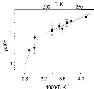
Figure 4. Comparison of experimental results and modeling with the Eley–Rideal mechanism: Experiments: ○, [HO 2 ] = 4 × 10 10 molecule/cm 3 ; ◆, [HO 2 ] = 4 × 10 10 molecule/cm 3 ; and ■ – [HO 2 ] = 5 × 10 11 molecule/cm 3 . Solid line: simulation of the experimental results at 240–300 K using an Arrhenius expression. Dashed line: Eley–Rideal modeling using the following parameters: f_1 = 0.2 , k_{\text{ads}} = c/4 ; A_{1\text{d}} = kT/h , \Delta H_{\text{ads1}} = 20 kcal/mol; A_{1\text{r}} = 3 \times 10^{-15} cm 3 /s; E_1 = -3 kcal/mol, Z = 6.4 \times 10^{14} molecule/cm 2 .
