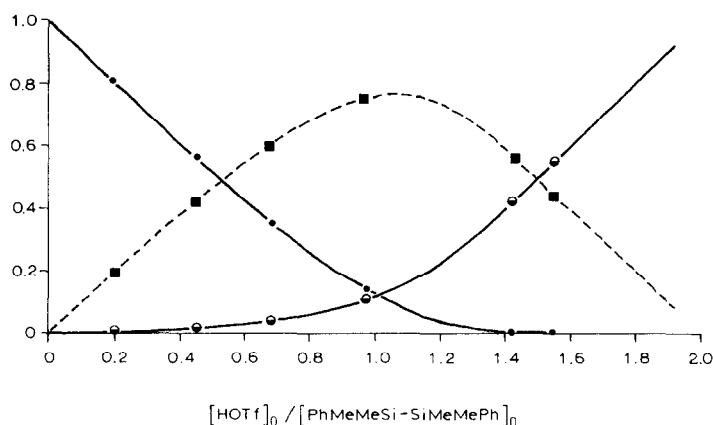
Fig. 1. Calculated (curves) and experimental proportions of 1,2-diphenyltetramethyldisilane (●), monotriflate (■) and ditriflate (⊖) at different [\text{acid}]_0/[\text{disilane}]_0 ratios. Calculations were performed assuming k_1/k_2 = 8 .
