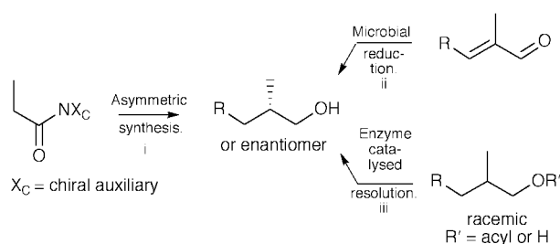
Scheme 1 Some examples of synthetic strategies for the preparation of enantiomerically pure 2-methylalkan-1-ols. Reagents and conditions: i, base then remove X c , then reduction; ii, baker's yeast reduction provides one enantiomer; iii, lipase catalysed kinetic resolution then product separation provides the pure enantiomers (one as ester).
