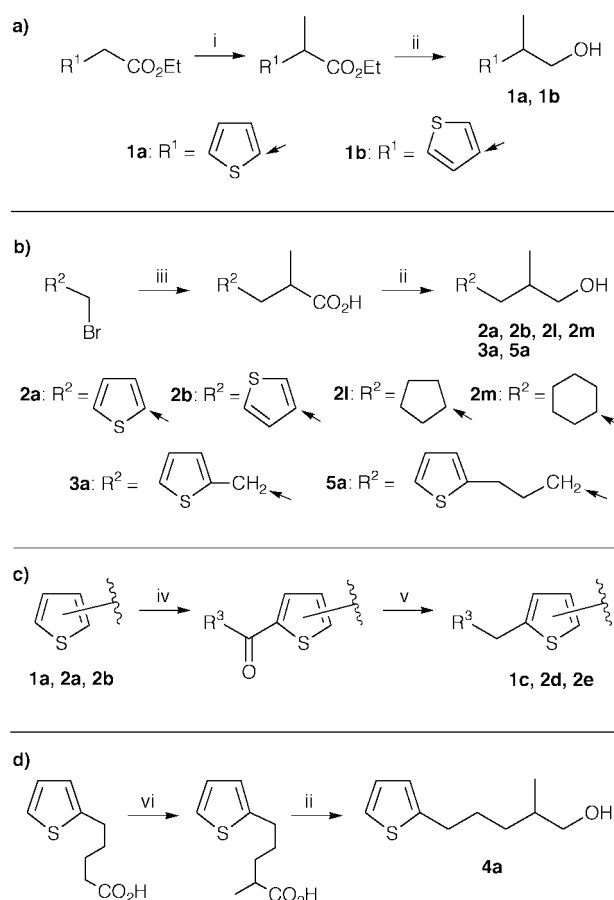
Scheme 2 Preparation of substrates containing thienyl and cycloalkyl moieties. For R^1 and R^2 , arrows indicate points of attachment. Reagents and conditions: i, LDA then MeI; ii, LAH then H_2O ; iii, Anion of diethyl methylmalonate then NaOH, EtOH, H_2O then H_3O^+ , H_2O then heat (decarboxylation); iv, R^3COCl , SnCl_4 , CH_2Cl_2 ; v, N_2H_4 , NaOH, diethylene glycol, 120 to >200^\circ C ; vi, 2 eq. LDA then MeOTf.
