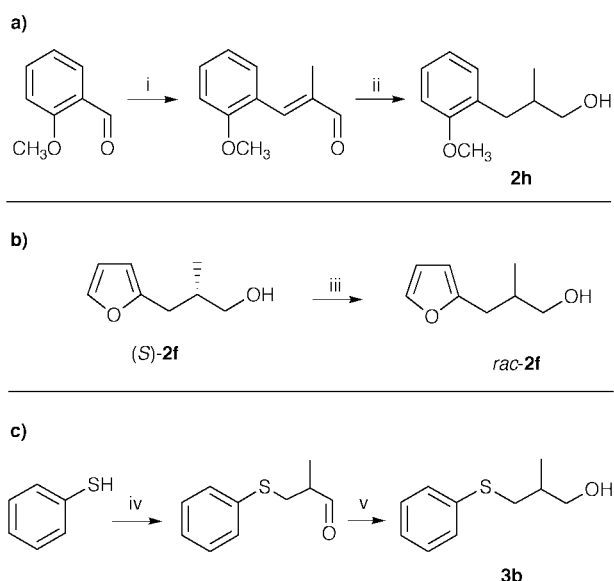
Scheme 3 Preparation of substrates without thienyl or cycloalkyl moieties. Reagents and conditions : i, Propanal, NaOH, EtOH, H 2 O; ii, Pd, H 2 then NaBH 4 ; iii, Na, toluene, reflux; iv, 2-methylprop-2-enal, Cupric acetate [catalyst]; v, NaBH 4 .
