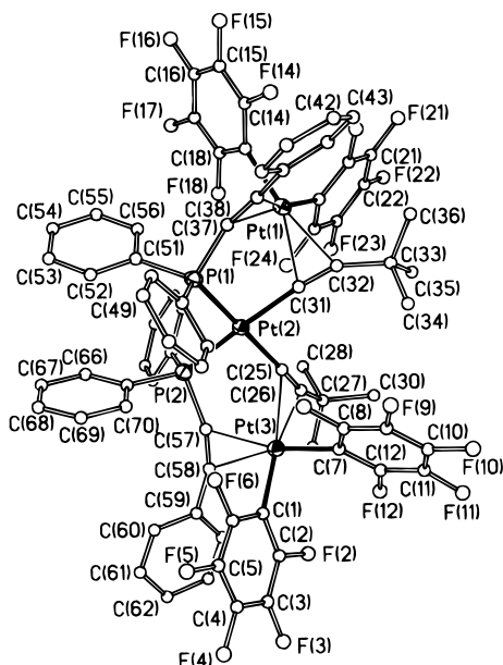
Figure 2. Drawing of the molecular structure of [\{\text{Pt}(\mu\text{-}\kappa(\text{P})\text{:}\eta^2\text{-PPh}_2\text{C}\equiv\text{CPh})_2(\mu\text{-}\eta^1\text{:}\eta^2\text{-C}\equiv\text{CBu}^1)_2\}\{\text{Pt}(\text{C}_6\text{F}_5)_2\}_2] , 15A .
