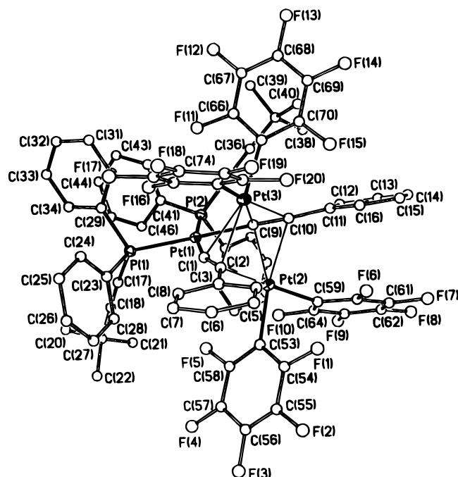
Figure 3. Molecular structure of [\{(\text{PPh}_2\text{C}\equiv\text{CBu}^1)_2\text{Pt}(\mu_3\text{-}\eta^2\text{-C}\equiv\text{CPh})_2\}\{\text{Pt}(\text{C}_6\text{F}_5)_2\}_2] , 16B .
