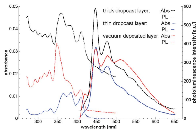
Fig. 4 Absorption (Abs) and photoluminescence (PL) spectra of thin films of L6P on quartz substrates, either prepared by vacuum deposition or drop-casting from \text{CH}_2\text{Cl}_2 solution.
