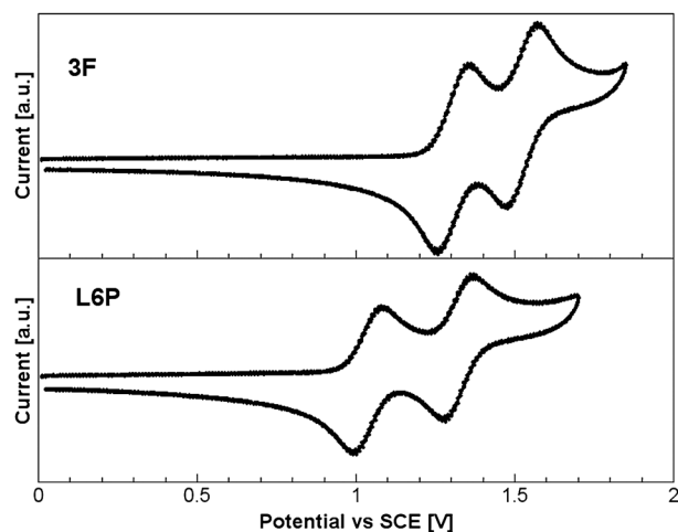
Fig. 2 Cyclic voltammogram of 3F (top) and L6P (bottom) in \text{CH}_2\text{Cl}_2 (0.1 M \text{Bu}_4\text{NPF}_6 ), dE/dt = 1 \text{ V s}^{-1} .
