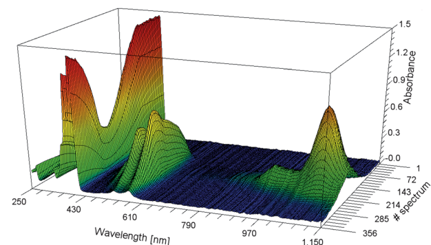
Fig. 3 Spectral change of L6P during electrochemical oxidation: formation of radical cation and dication ( c = 8 \times 10^{-5} \text{ M}^{-1} in \text{CH}_2\text{Cl}_2 ). Recorded in a 1 mm quartz cuvette using a platinum grid electrode, 0.1 M \text{Bu}_4\text{NPF}_6 , dE/dt = 10 \text{ mV s}^{-1} , 0 \rightarrow 1.3 \rightarrow 0 \text{ V} vs. \text{Ag}/\text{AgNO}_3 , spectra recorded every 7.3 mV.
