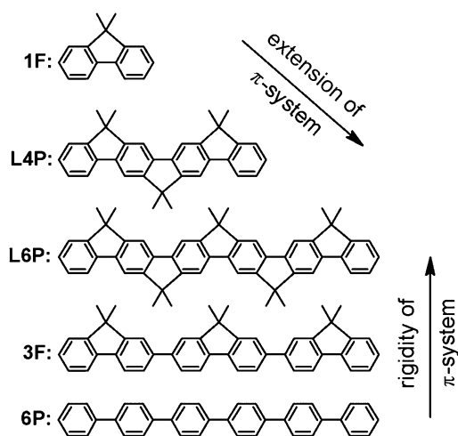
Scheme 3 Characterized compounds and variation of their structural parameters.
