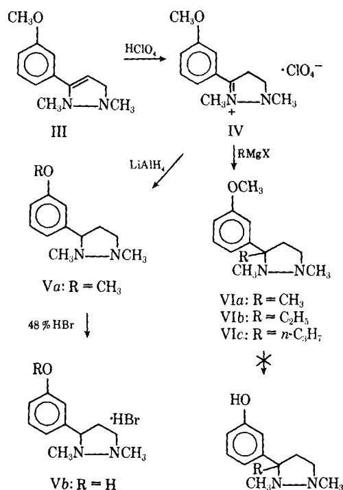
Scheme I
