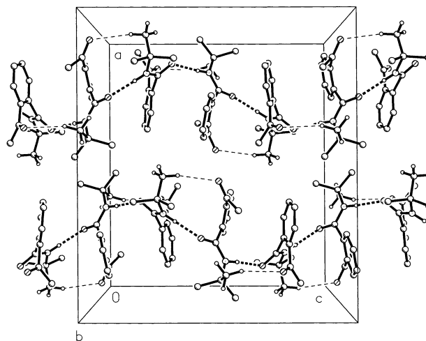
Figure 6. Packing diagram of 8 , showing helical chains of molecules (related by the a 1 operator) connected by hydrogen bonds (dashed lines). Only H atoms involved in H bonds, together with their geminal neighbors, are included. The partially occupied water site (see text) is omitted. View direction parallel to the z axis.
