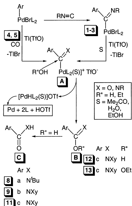
Scheme 6
