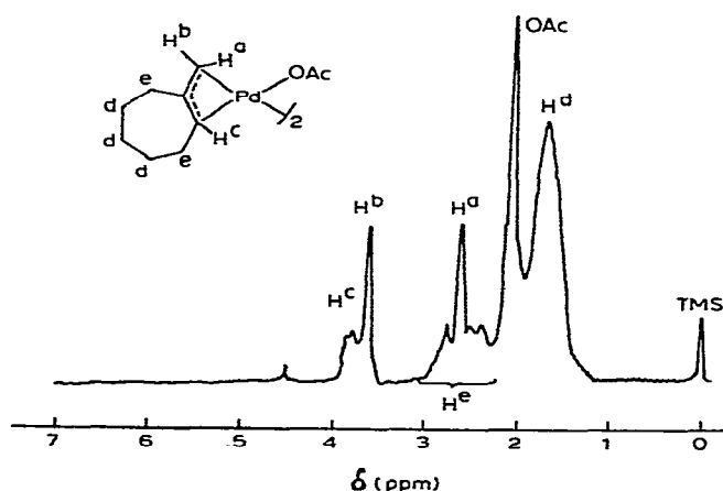
Fig. 2. NMR spectrum of reaction mixture of methylenecyclopentane with \text{Pd}(\text{OAc})_2 concentrated under vacuum.
