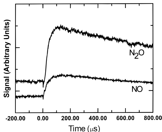
Figure 1. Transient infrared absorption signals for \text{N}_2\text{O} and NO product molecules. Probed lines are NO \nu = 0 R(4.5) and \text{N}_2\text{O} ( 00^0 0 ) P(23). Reaction conditions are the following: P_{\text{ICN}} = 0.05 , P_{\text{NO}_2} = 0.05 , P_{\text{NH}_3} = 1.0 , and P_{\text{SF}_6} = 1.0 Torr.
