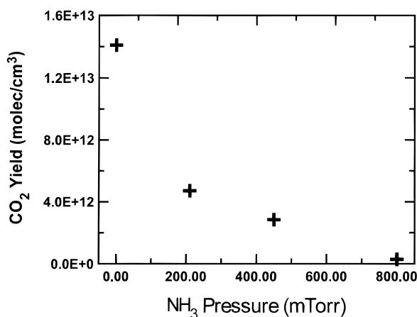
Figure 3. CO 2 product yields as a function of NH 3 pressure. Reaction conditions are the following: P_{\text{ICN}} = 0.03 , P_{\text{NO}_2} = 0.05 , P_{\text{NH}_3} = variable, and P_{\text{SF}_6} = 1.0 Torr.
