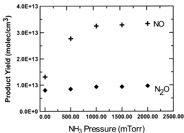
Figure 2. N 2 O and NO product yields as a function of NH 3 pressure. Reaction conditions are the following: P_{\text{ICN}} = 0.05 , P_{\text{NO}_2} = 0.05 , P_{\text{NH}_3} = variable, and P_{\text{SF}_6} = 1.0 Torr.
