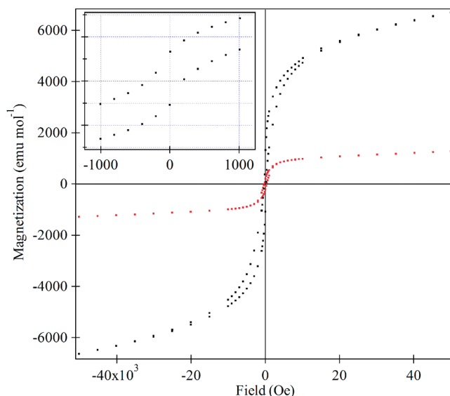
Figure 6. Magnetization-field isotherms collected at 300 K (red) and 5 K (black) from \text{Sr}_3\text{FeCoO}_4\text{Cl}_2 . Inset shows an expanded region of the 5 K isotherm emphasizing that the data are displaced to higher magnetizations.
