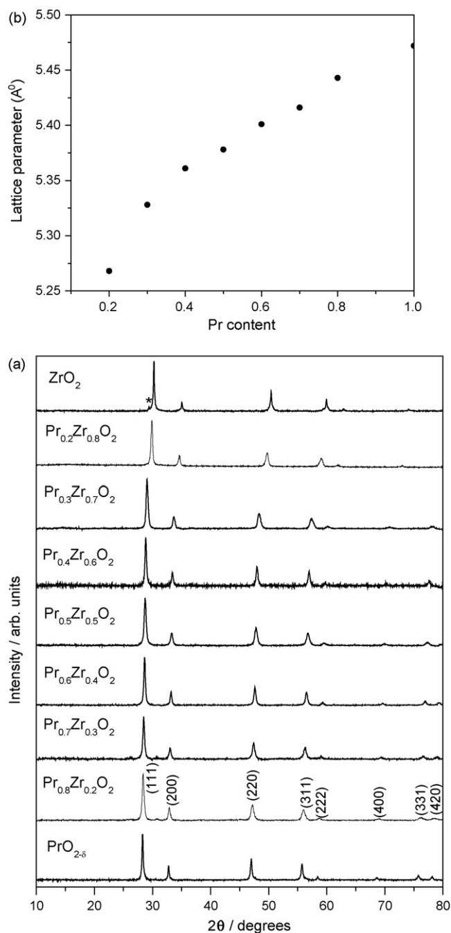
Fig. 1. (a) Powder XRD pattern of \text{Pr}_{1-x}\text{Zr}_x\text{O}_{2-\delta} ( 0 \leq x \leq 1 ) (in \text{ZrO}_2 , asterisk indicates monoclinic impurity phase). (b) Plot of lattice parameter 'a' vs. composition of Pr.
