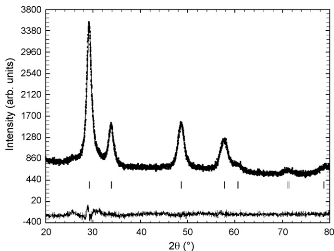
Fig. 3. Rietveld refined XRD pattern of \text{Pr}_{0.48}\text{Pd}_{0.02}\text{Zr}_{0.5}\text{O}_{1.898} .
