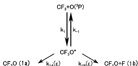
Figure 3. Model for the product channels of the CF 3 + O( 3 P) reaction used in the calculation of branching fractions.
