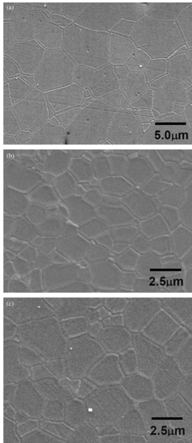
Fig. 5. Scanning electron microscopy images of the alumina ( \text{Al}_2\text{O}_3 ) ceramics that were spark plasma sintered at (a, c) 1350°C and (b) 1300°C, using (a) the untreated and (b, c) the pretreated \text{Al}_2\text{O}_3 powder. The bright spots on image (a) and (c) are contaminant particles that fell on the sample surface during the thermal etching process.
