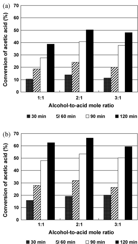
Fig. 3. Effect of mole ratio on the esterification of acetic acid with n -Butanol using 5V-Al 2 O 3 (a) and 10V-Al 2 O 3 (b) as catalysts. Reaction conditions: temperature 100 °C, 0.7 wt % catalyst.
