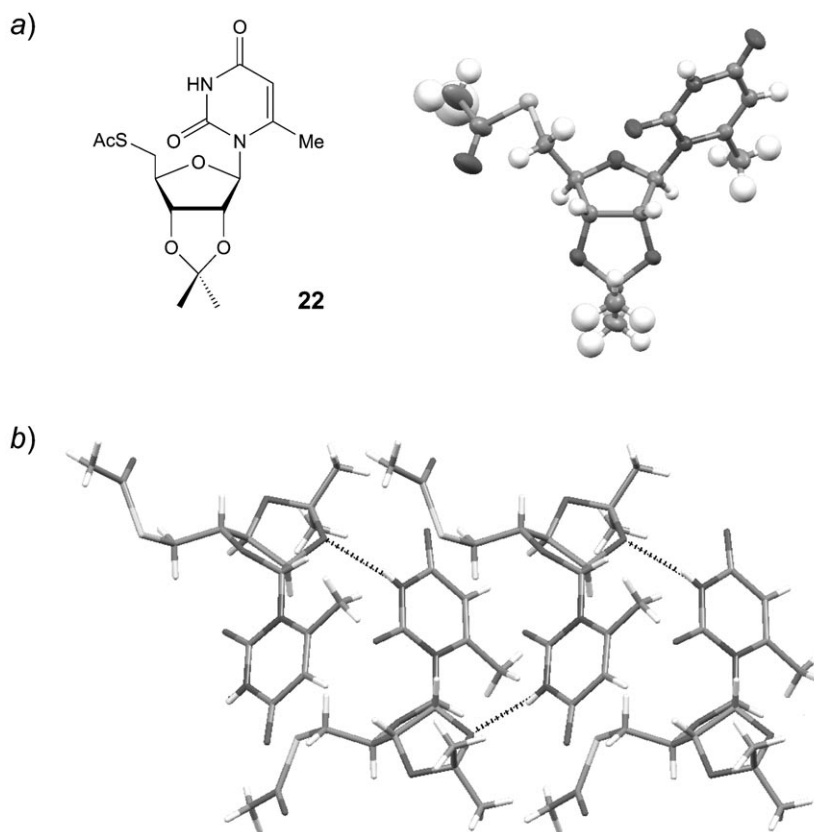
Fig. 1. Crystal structure of 22 . a) ORTEP Representation. b) Molecular packing showing intermolecular N(3)–H...O(2') H-bonds (hashed bonds).
