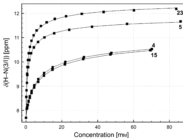
Fig. 2. Shift/concentration curves (SCCs) for the A^*[s]U^{(3)} dimers 4 , 5 , 15 , and 23 in CDCl_3 solution (including a value of 7.70 ppm for a 0.0001-M soln.)
