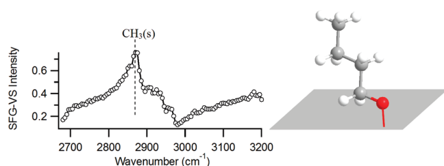
Figure 5. SFG-VS reference spectrum of 1 Torr of butanol over Pt(111) at 23 °C. The dominant \text{CH}_3(\text{s}) peak at 2875 \text{cm}^{-1} indicates that butanol adsorbs upright on the surface.
