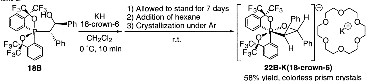
Scheme 17
