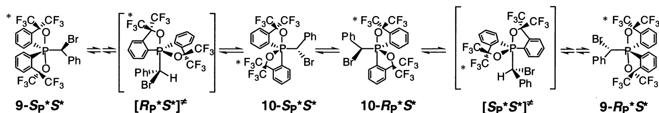
Scheme 10
