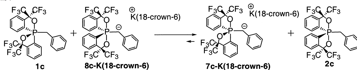
Scheme 7
