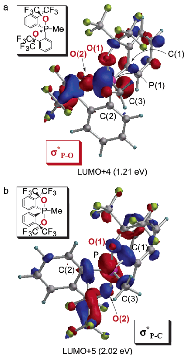
Figure 3. Calculated molecular orbitals and the energies of \sigma^*_{\text{P-O}} orbital in 1 and \sigma^*_{\text{P-C}} orbital in 2 , which should be responsible for the difference in the nucleophilic attack.
