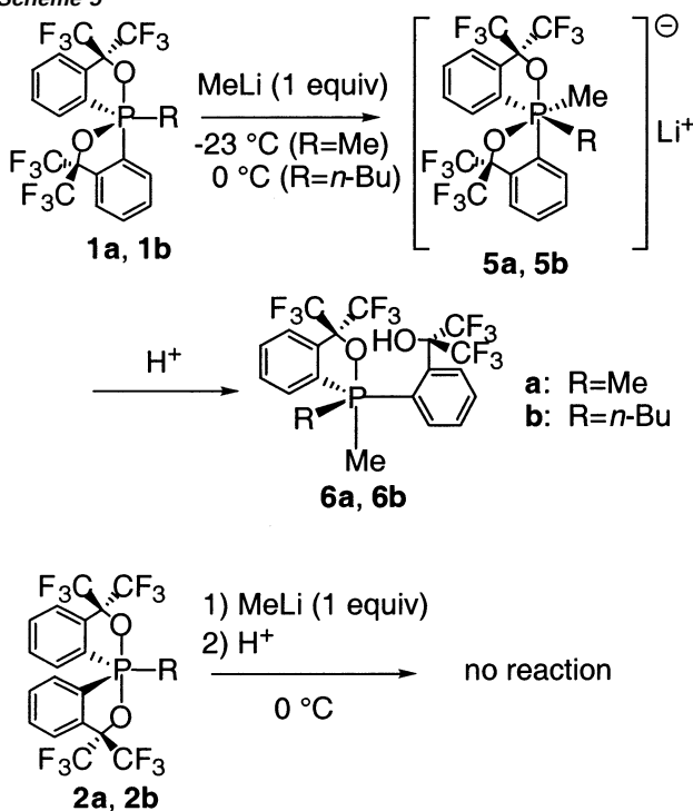
Scheme 5
