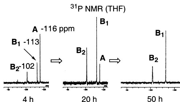
Figure 7. Time course of the ^{31}P NMR signals of the reaction of 7c-Li with PhCHO .
