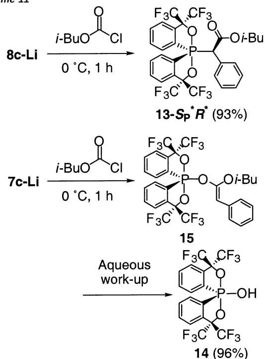
Scheme 11
