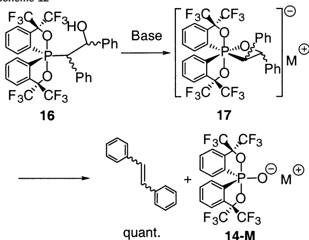
Scheme 13
