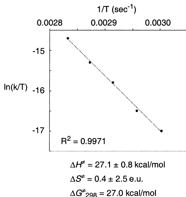
Figure 12. Eyring plot of the rate constants for the thermal decomposition of 22B-K(18-crown-6) .
