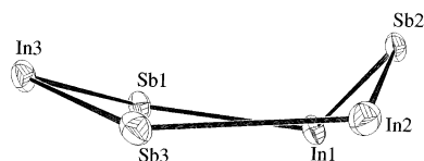
Fig. 2. ORTEP diagram (30% probability ellipsoids), side view, showing the distorted twist-boat conformation of [\text{Et}_2\text{InSb}(\text{SiMe}_3)_2]_3 ( 1 ). Silicon, carbon, and hydrogen atoms are omitted for clarity.
