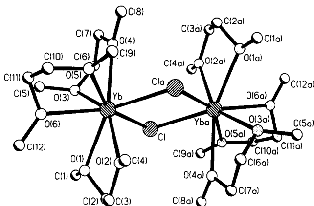
Fig. 1. The structure of the [\text{Yb}(\text{DME})_3\text{Cl}]_2^+ cation.
