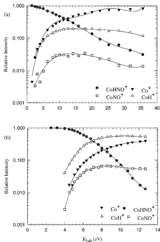
Figure 6. Energy-resolved CID (a) and SORI-CID (b) breakdown curves of \text{CoHNO}^+ .
