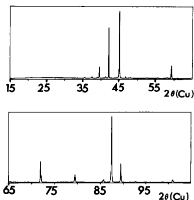
Fig. 6. X-ray diffraction patterns of \text{Cu}_5\text{Ge} (molar ratio of 0.45).
