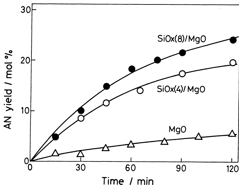
Fig. 2. Formation of acetonitrile over \text{SiOx/MgO} catalyst.
