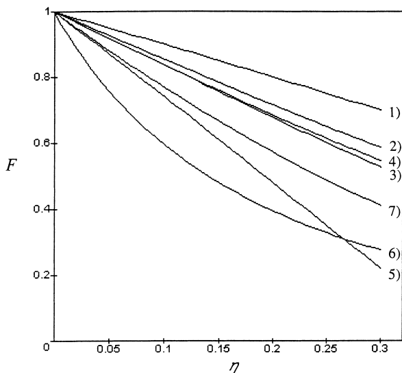
Figure. Correction factor F as a function of the porosity \eta . The numbers on the right-hand side of the graphs indicate the correction functions namely: (1) simple linear correction; (2) correction with spherical pores; (3) correction with open porosity with randomly distributed pores angles ( \cos^2\psi=1/3 ); (4) correction based on finite-element calculus for a \text{UO}_2 material. The graph just shows the curve calculated with the intermediate exponent value 1.7 (without the range \pm 0.2 ); (5) empirical correction (modified Loeb), with \xi=2.6-0.5 \times 10^{-5}T ( T=20 , temperature in ^{\circ}\text{C} ) [20]; (6) Maxwell–Eucken correction, with \beta=6.5-0.00469T ( T=291 , temperature in \text{K} ) [21]; and (7) correction derived from points (5) and (6).
