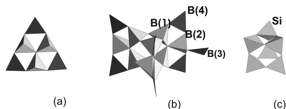
Figure 1. Structural blocks: isolated hexaborate block 6:[3\text{T}+3\Delta] = [\text{B}_6\text{O}_7(\text{OH})_6]^{2-} (a); complex double hexaborate ring 3\times\{6:[3\text{T}+3\Delta]-1\Delta\} = [\text{B}_{15}\text{O}_{24}(\text{OH})_6]^{9-} of B(1), B(2), and B(4) polyhedra with additional B(3) triangle for condensation into the layer (b); double “dreier” ring 6:[6\text{T}] = [\text{Si}_6\text{O}_{15}]^{6-} in Na,Y-silicate (c).
