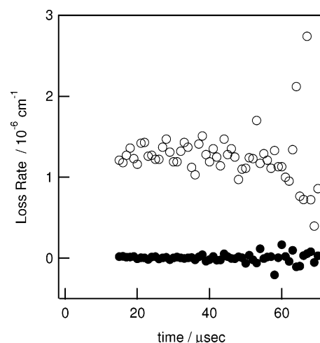
Figure 3. Temporal profile of the cavity loss rate measured in the presence of NO 3 (empty circles) and the empty cavity loss rate (dark circles). Individual data are the result of the photolytic differencing procedure described in the text.
